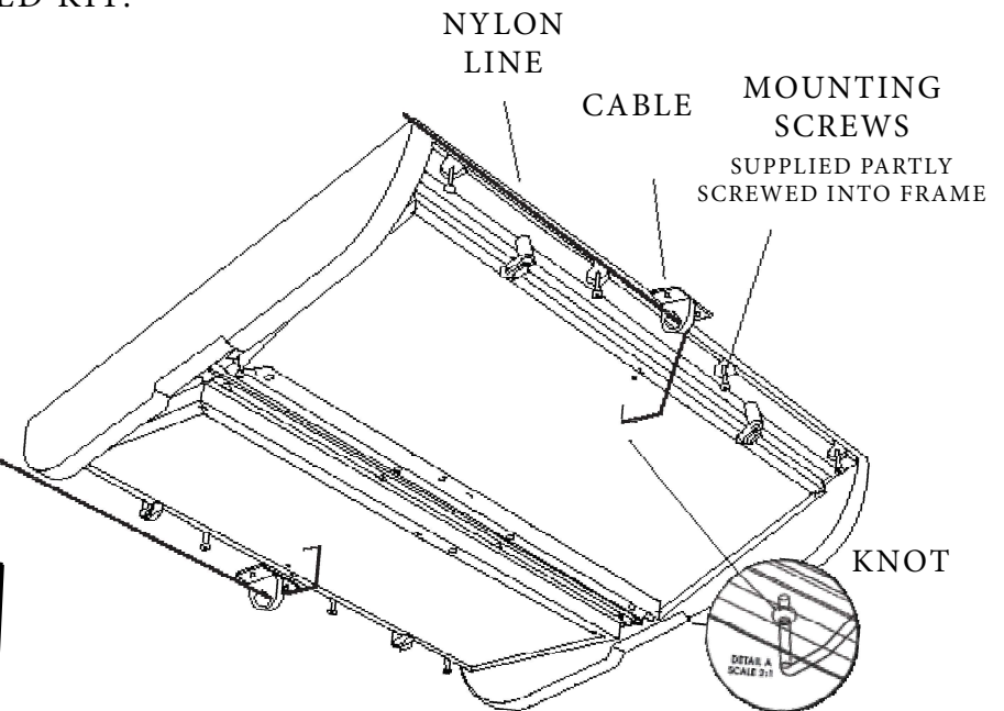
#10 x 1 1/2" SCREWS
