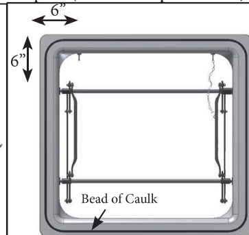
Step 3: (Caulk Top of Inlet)
