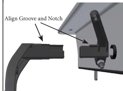
Step 6: (Weight Arm)
