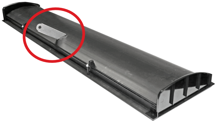
CSW INLET WITH SPLIT BOLT AND NUT
