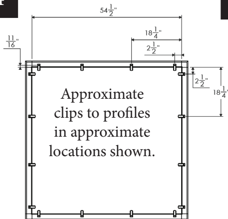
Install extension with clips.
