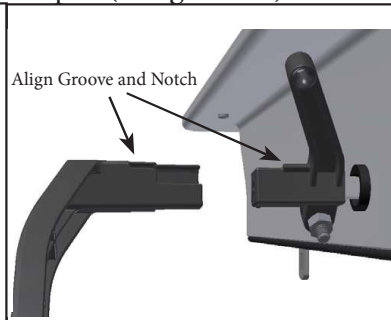
Step 6: (Weight Arm)
