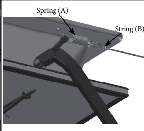
Step 8: (Shut-off)
