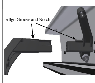
Step 6: (Weight Arm)
